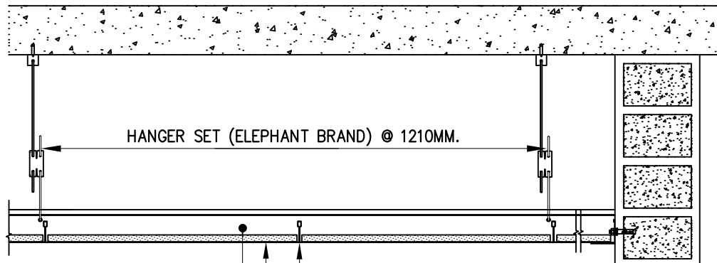
SECTION 1-1 SCALE 1 : 7.5
