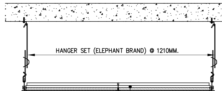
SECTION 2-2 SCALE 1 : 7.5
