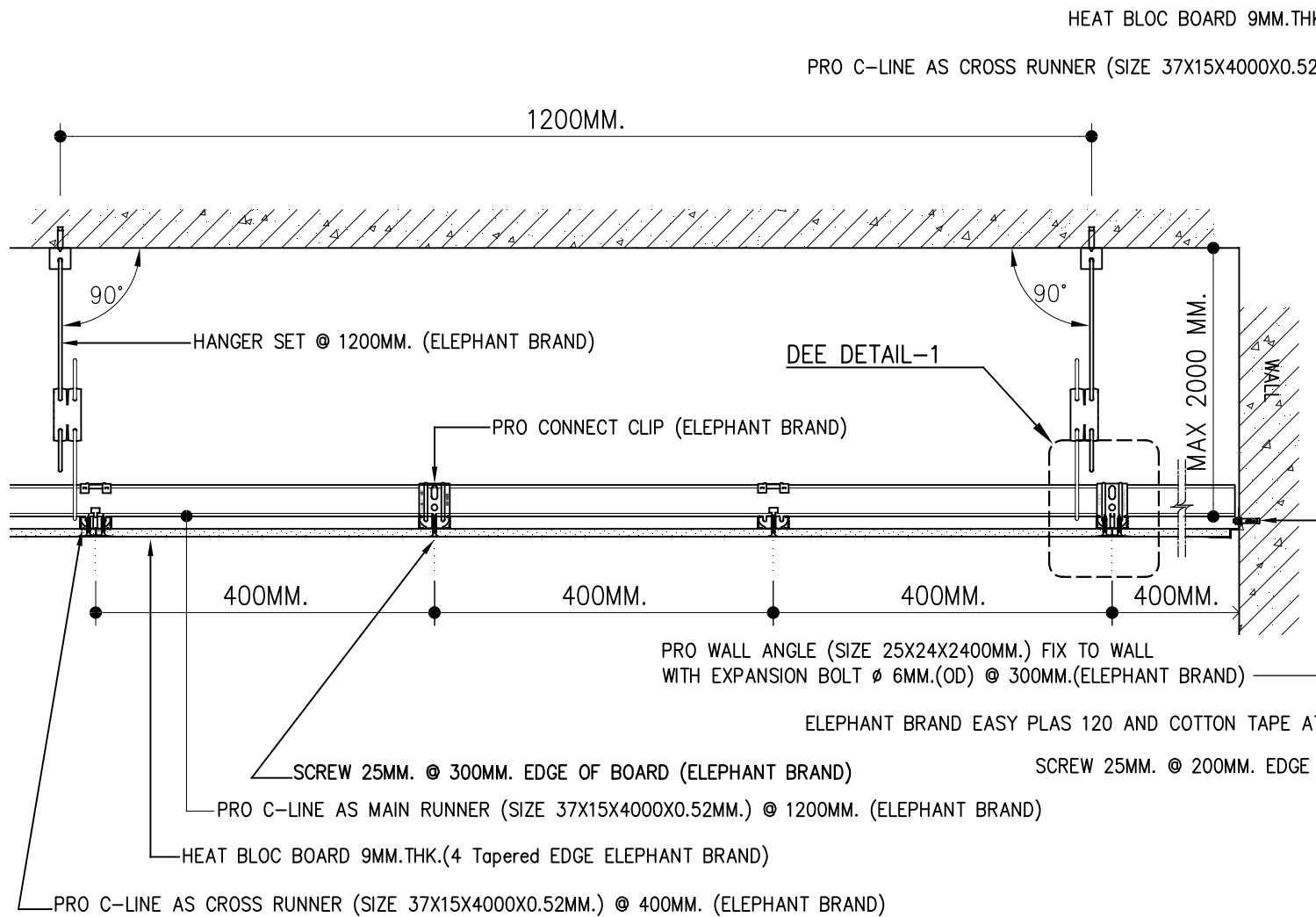
SECTION-A SCALE 1 : 8
