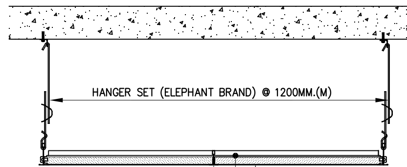
SECTION 2-2 SCALE 1 : 7.5
