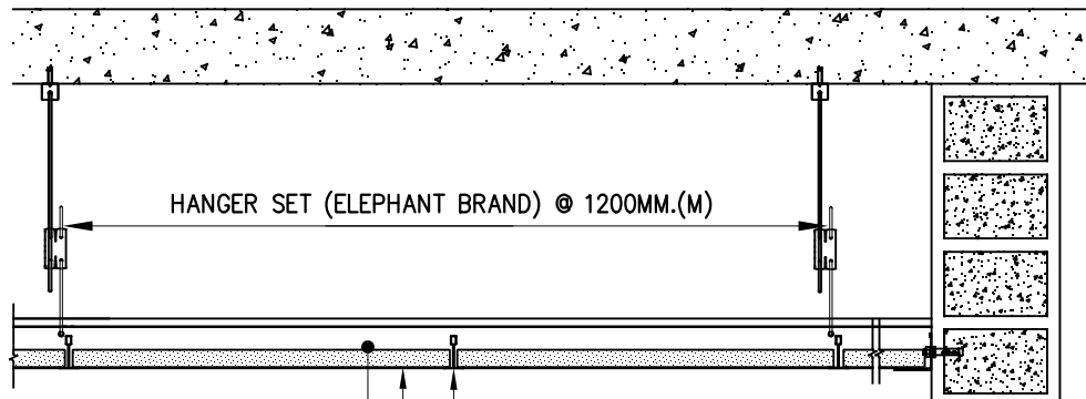
SECTION 1-1 SCALE 1 : 7.5
