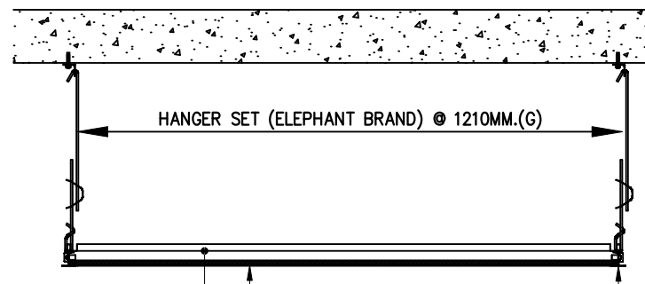
SECTION 2-2 SCALE 1 : 7.5
