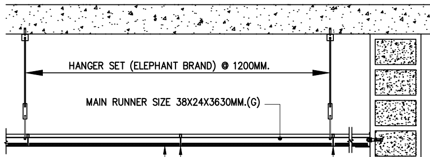
SECTION 1-1 SCALE 1 : 7.5
