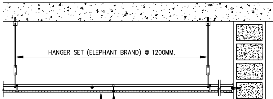
SECTION 1-1 SCALE 1 : 7.5
