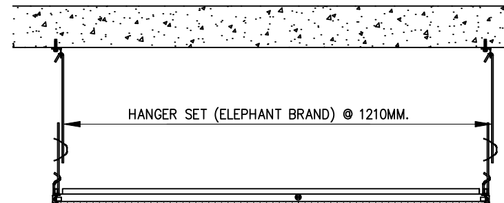
SECTION 2-2 SCALE 1 : 7.5
