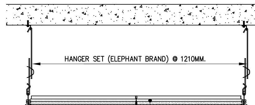
SECTION 2-2 SCALE 1 : 7.5
