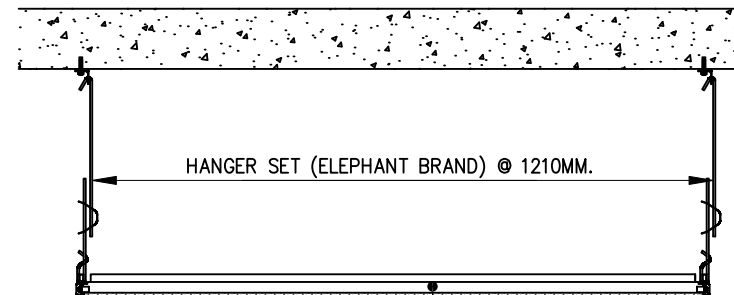
SECTION 2-2 SCALE 1 : 7.5
