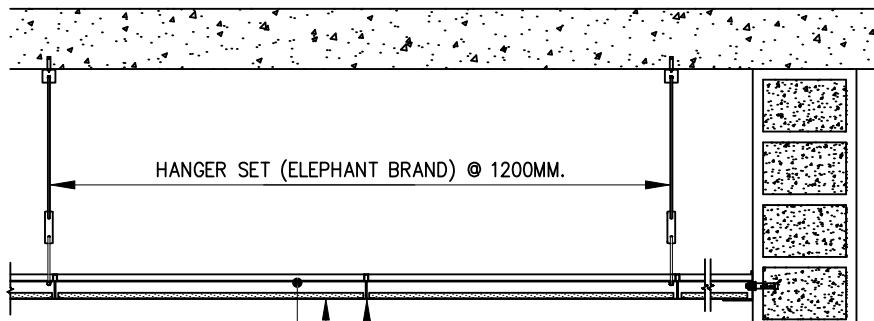
SECTION 1-1 SCALE 1 : 7.5
